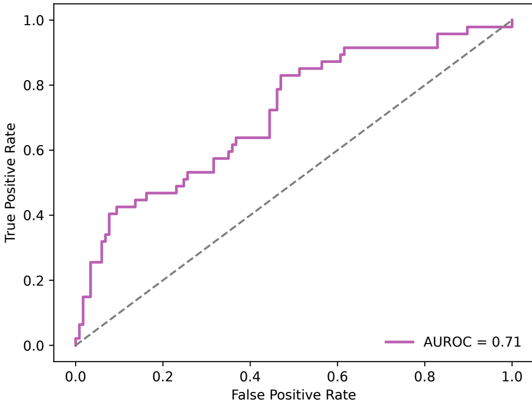
NB ROC Curve
